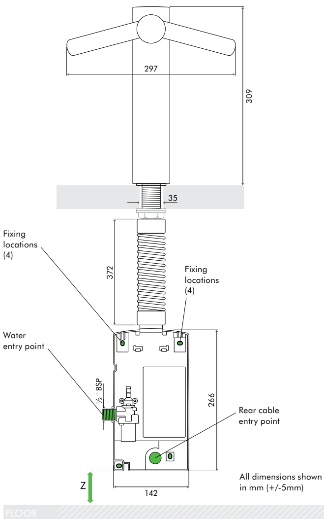
REAR ELEVATION
