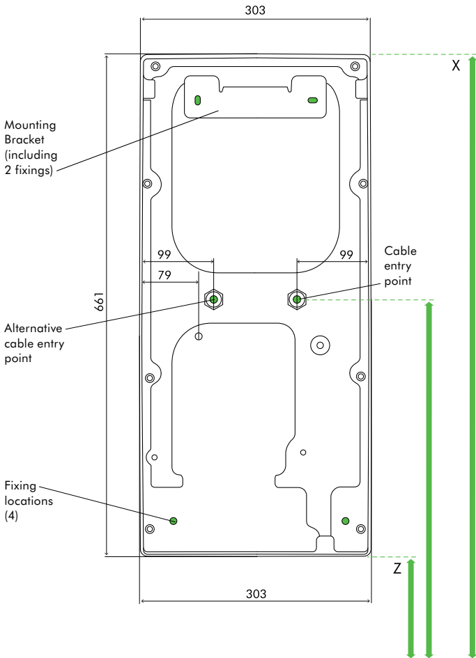
REAR ELEVATION
