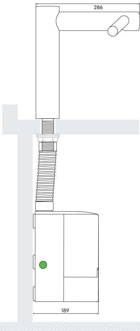
SIDE ELEVATION
