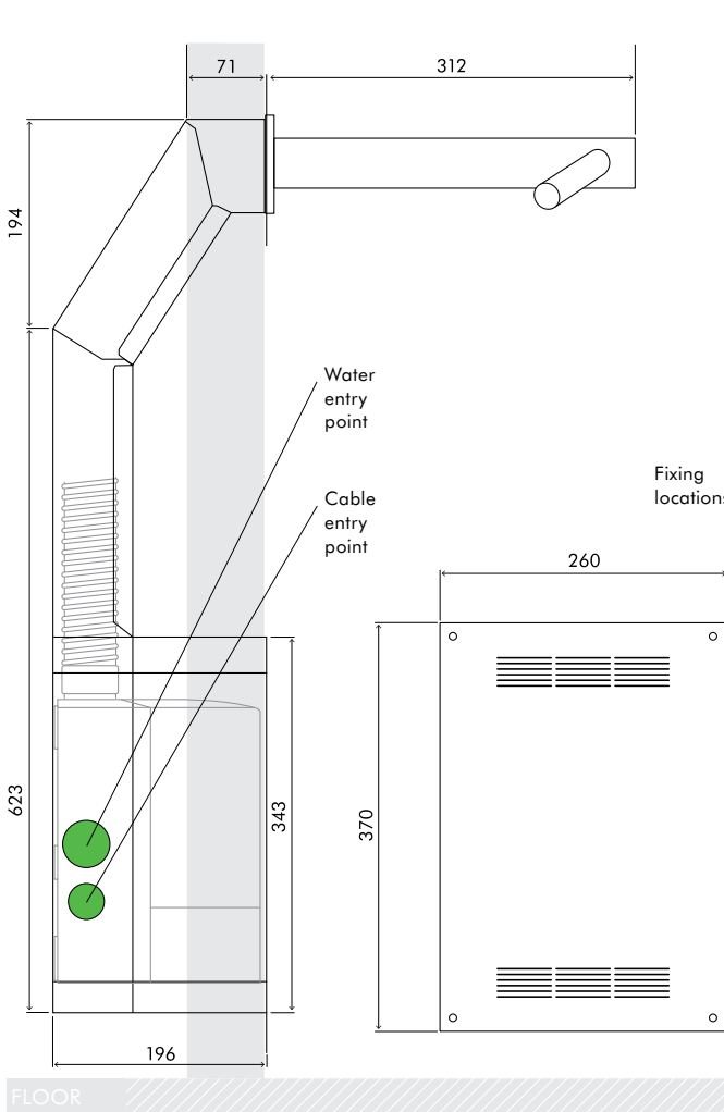
SIDE ELEVATION
