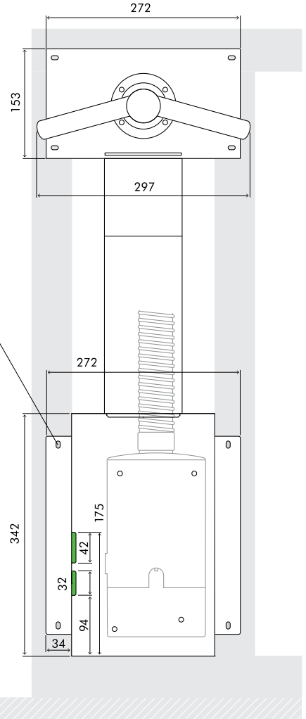
REAR ELEVATION
