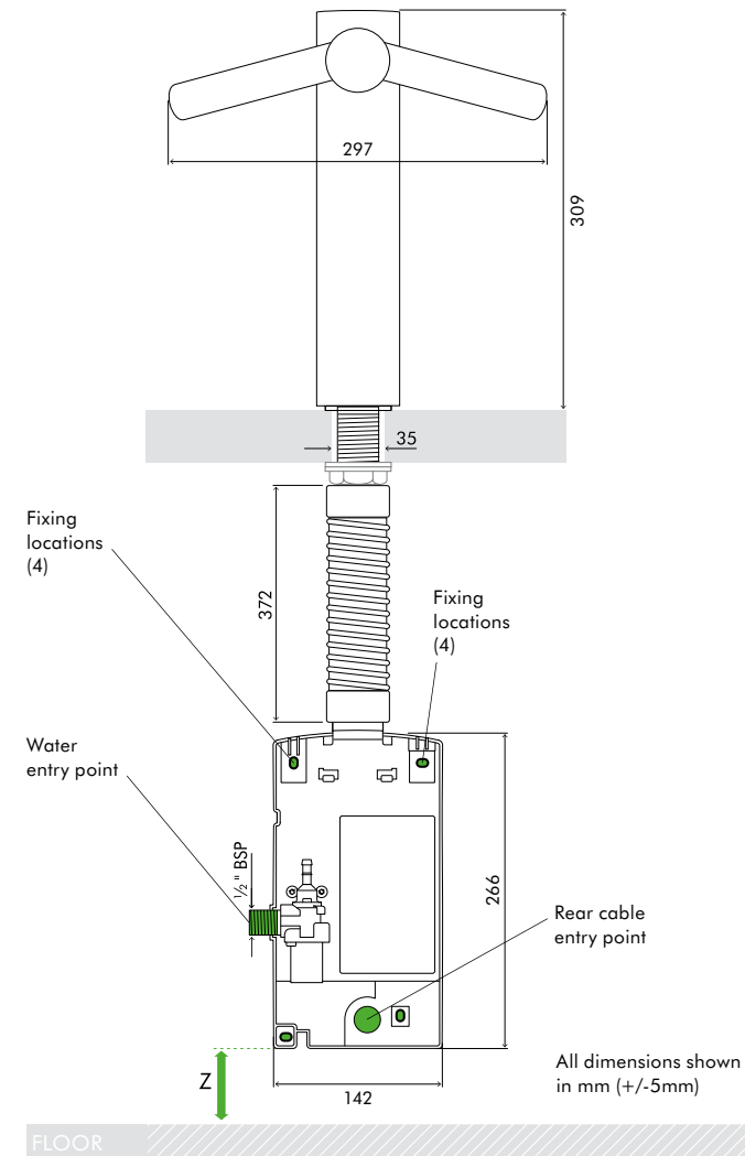
REAR ELEVATION
