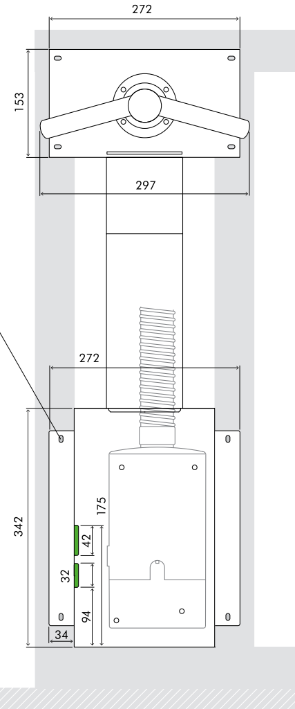
REAR ELEVATION
