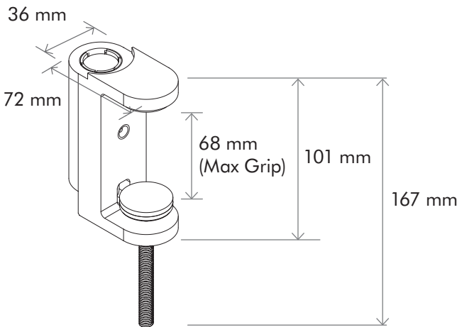
CLAMP MECHANISM
